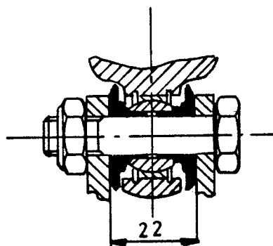
DETAIL ①
