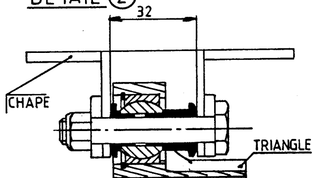
DETAIL ②
